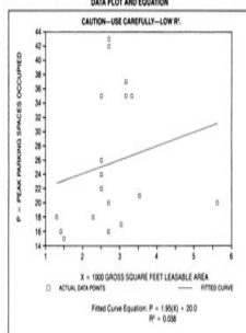
Fig. 2. Parking generation at fast food restaurants with drive-in windows. Source: Institute of Transportation Engineers (1987a, p. 146).
