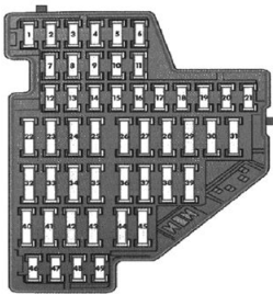
Volkswagen Golf 5 - fuse box passenger compartment
